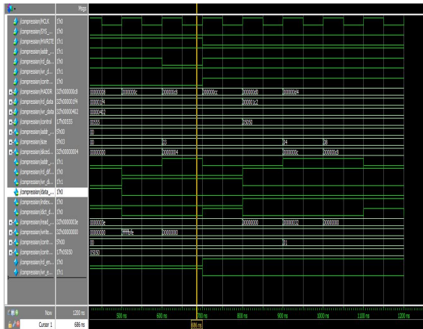
Fig 5. Simulation result of compression module
