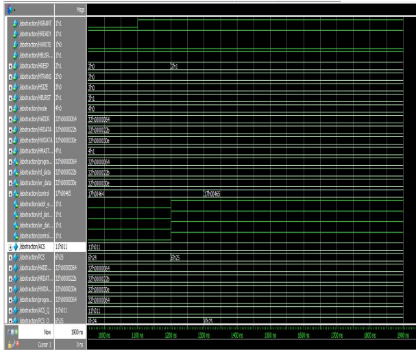
Fig 4. Simulation result of abstraction module
