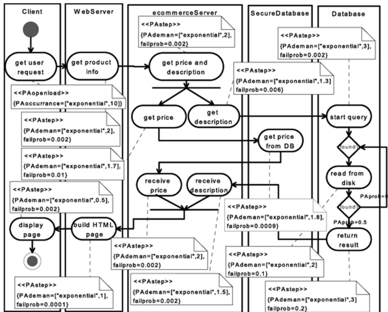
Figure 6. Annotated Activity Diagram for products information display
